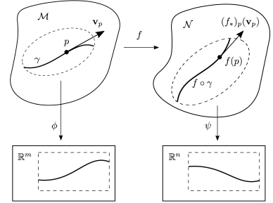
Pushforward of a vector field
